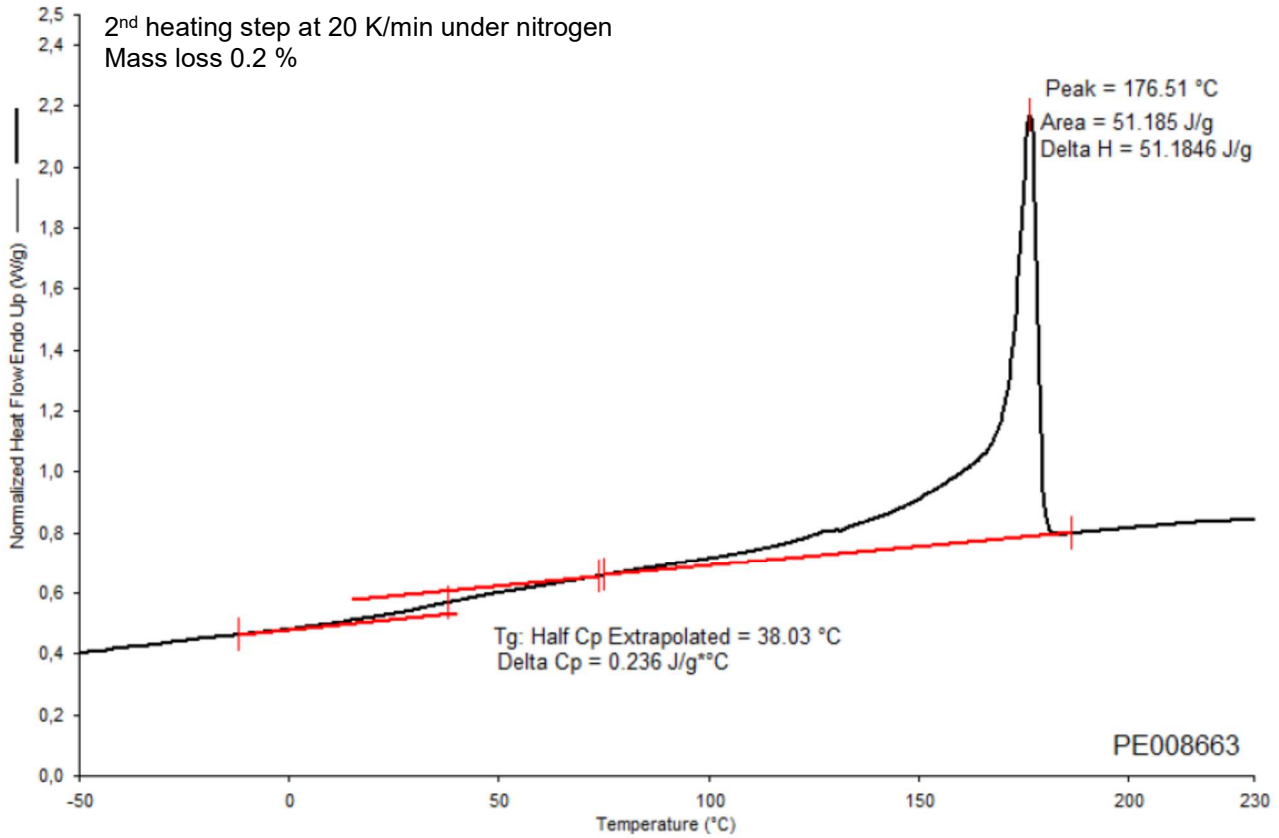
Figure B.1: Determination of the melting point during the second heating step
